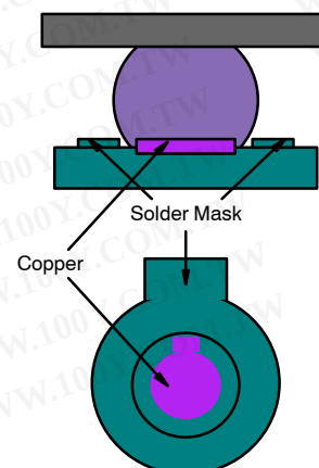
FIGURE 4. NSMD
