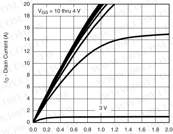
V_{GS} = 10 thru 4V Output Characteristics
