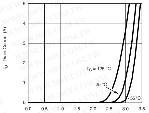
T_C = 125^\circ C 25^\circ C -55^\circ C Transfer Characteristics
