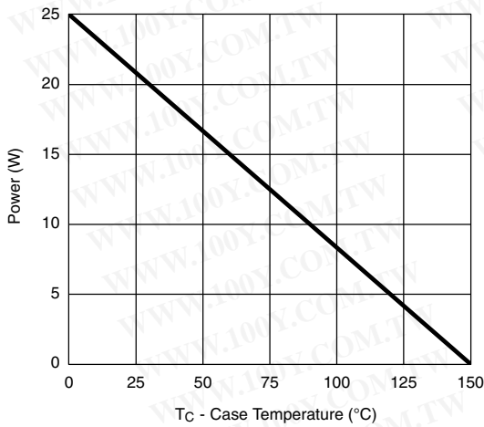
T_C - Case Temperature (°C) Power, Junction-to-Case
