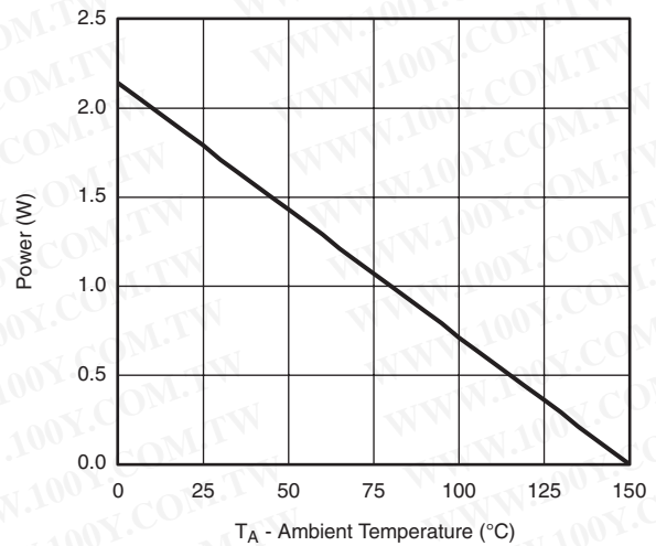
T A - Ambient Temperature (°C) Power Junction-to-Ambient
