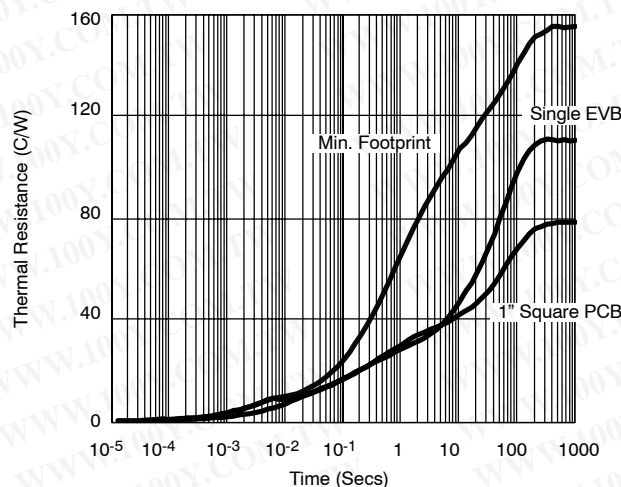
FIGURE 4. Single 1206-8 ChipFET
