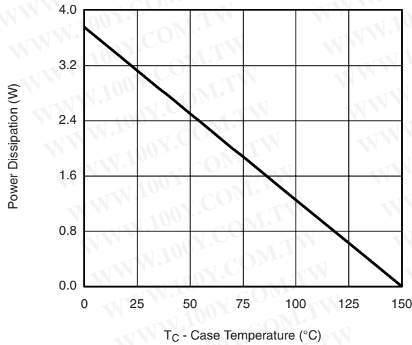
T c - Case Temperature (°C) Power Derating, Junction-to-Foot
