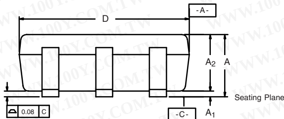
5-LEAD TSOP
