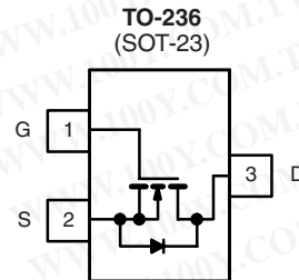
Top View Si2304BDS (L4)*
