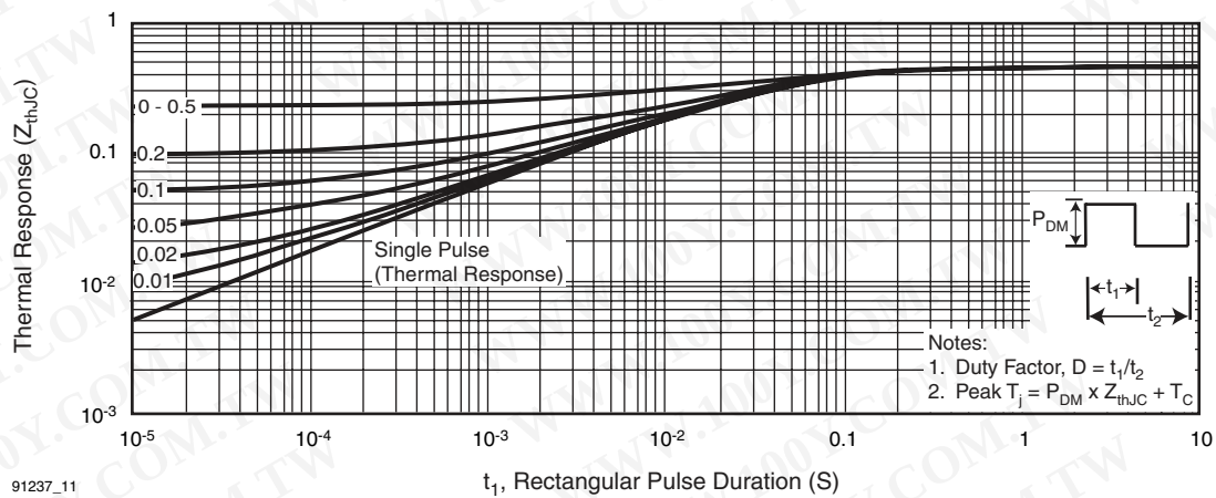
Fig. 11a - Maximum Effective Transient Thermal Impedance, Junction-to-Case
