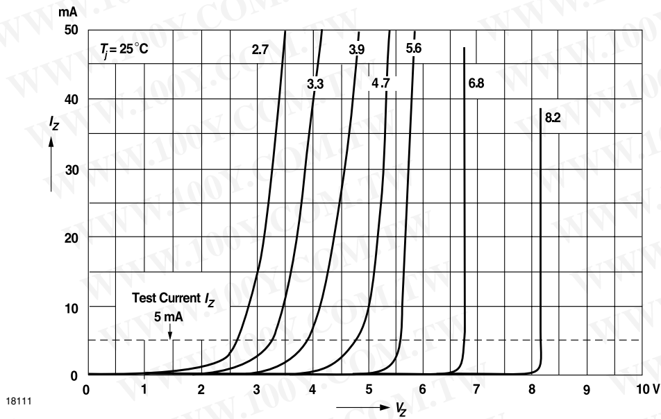
Figure 16. Breakdown Characteristics
