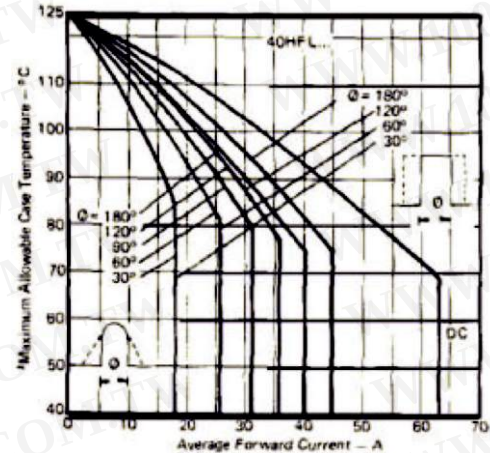
Fig. 14 - Average Forward Current vs. Maximum Allowable Case Temperature, 40HFL Series
