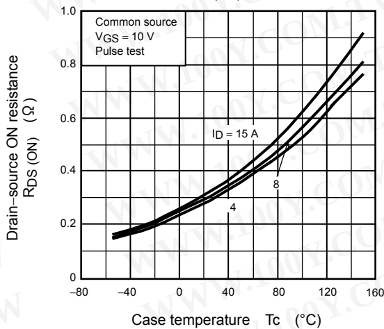
R_{DS(ON)} - T_c
