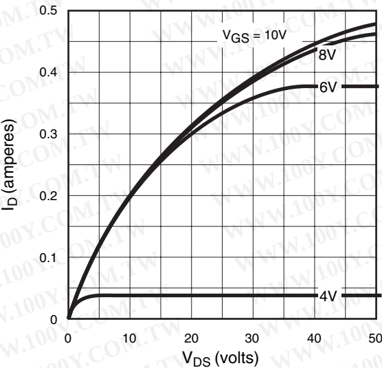
Output Characteristics
