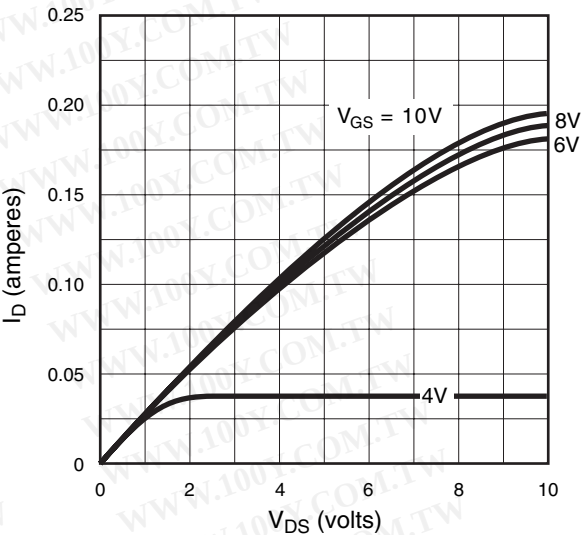
Saturation Characteristics
