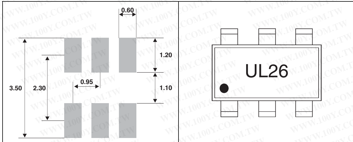
Figure 22. SOT23-6L footprint dimensions in mm
