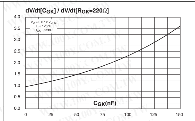
Figure 10. Relative variation of dV/dt immunity versus gate-cathode capacitance (typical values) for TS12 series
