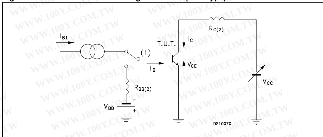
Figure 2. Resistive load switching test circuit (NPN type)
