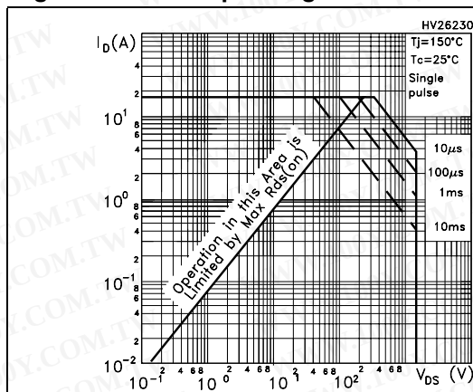
Figure 4. Safe operating area for TO-3PF
