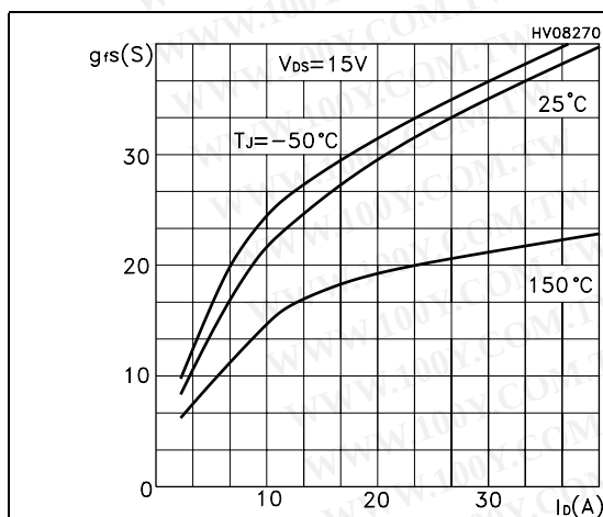
Figure 5. Transconductance
