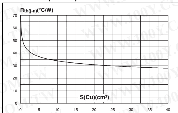
Figure 13. Thermal resistance junction to ambient versus copper surface under tab (epoxy FR4, e_{Cu} = 35 \mu\text{m} ) ( D^2\text{PAK} )
