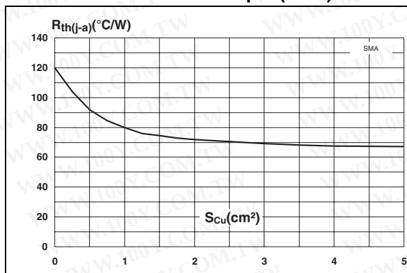
Figure 15. Thermal resistance junction to ambient versus copper surface under each lead - epoxy printed circuit board FR4, copper thickness = 35 \mu\text{m} (SMA)
