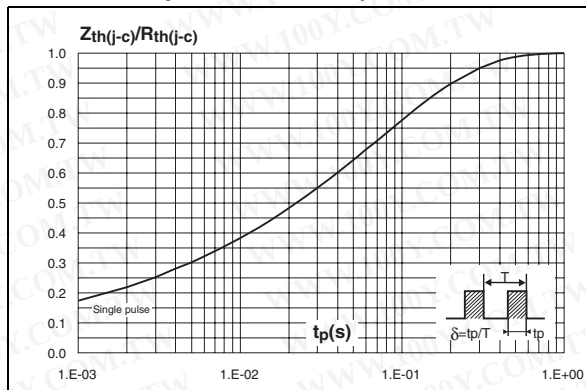
Figure 7. Relative variation of thermal impedance junction to case versus pulse duration (TO-220AB & I 2 PAK)
