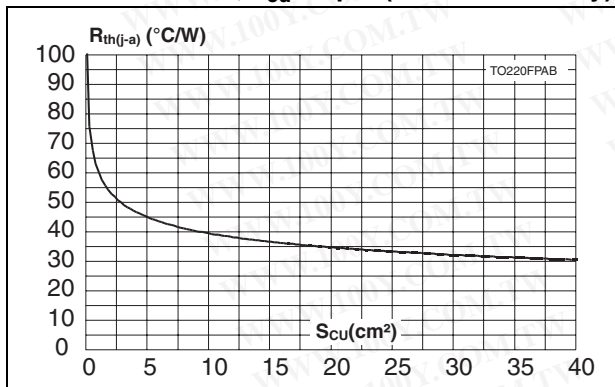
Figure 13. Thermal resistance, junction to ambient, versus copper surface under tab - Epoxy printed circuit board, e cu 35 μm (TO220FPAB only)
