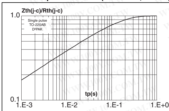
Figure 7. Relative variation of thermal impedance junction to case versus pulse duration (TO-220AB, D 2 PAK)
