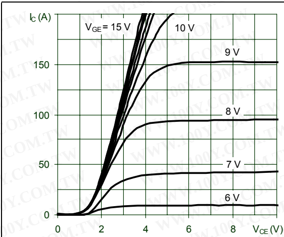
Figure 2. Output characteristics
