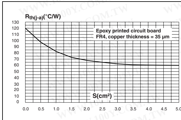
Figure 15. Thermal resistance junction to ambient vs. copper surface under tab P010xxN
