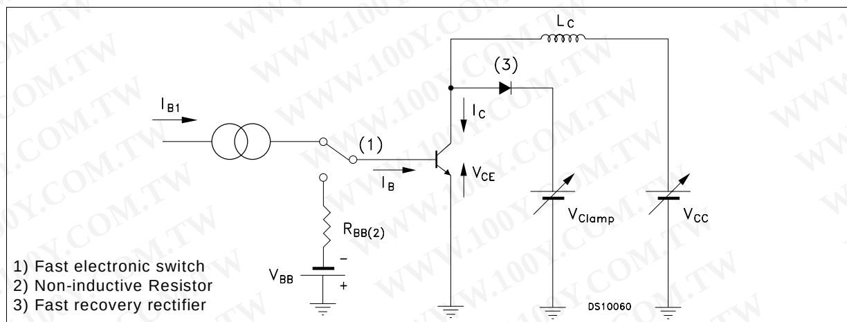
Inductive Load Switching Test Circuit
