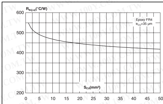
Figure 7. Thermal resistance junction to ambient versus copper surface under each lead (SOD-323)
