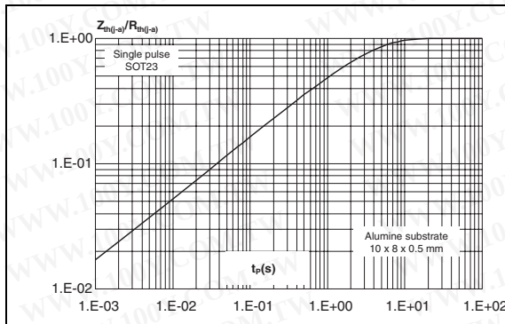
Figure 9. Relative variation of thermal impedance junction to ambient versus pulse duration (SOT-23)
