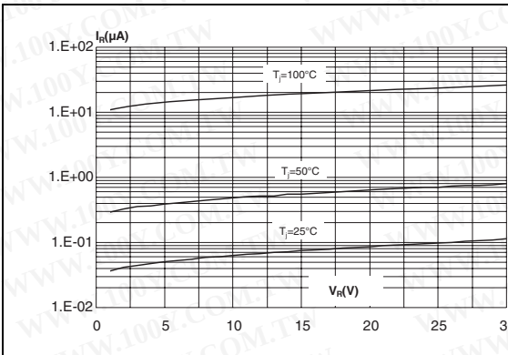
Figure 3. Reverse leakage current versus reverse applied voltage (typical values)
