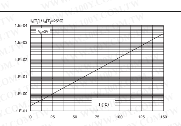
Figure 4. Reverse leakage current versus junction temperature
