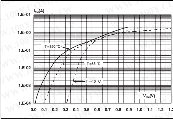
Figure 13. Forward voltage drop versus forward current (typical values)
