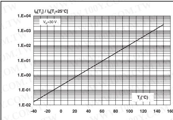
Figure 11. Relative variation of reverse leakage current versus junction temperature (typical values)
