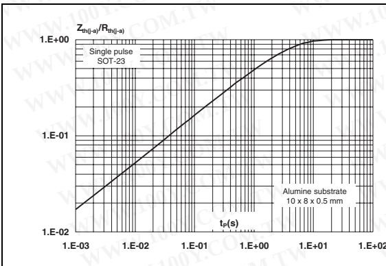
Figure 3. Relative variation of thermal impedance junction to ambient versus pulse duration
