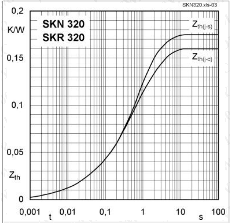
Fig. 4 Transient thermal impedance vs. time
