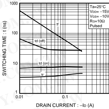
Fig.2 Switching Characteristics
