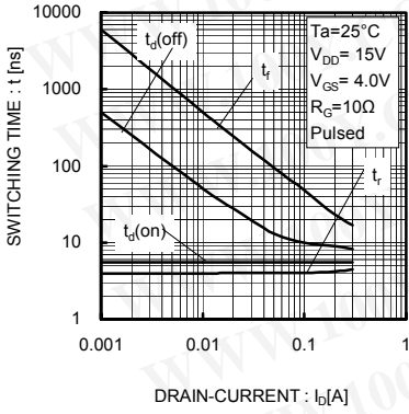
Fig.10 Switching Characteristics
