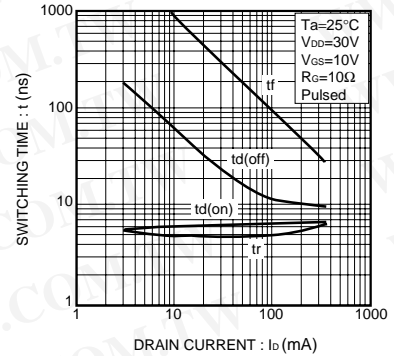
Fig.12 Switching Characteristics
