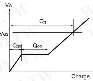
Fig.14 Gate Charge Waveform
