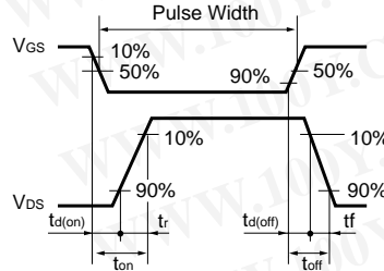
Fig.3-2 Switching Waveforms
