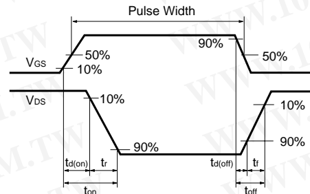
Fig.14 Switching Waveforms
