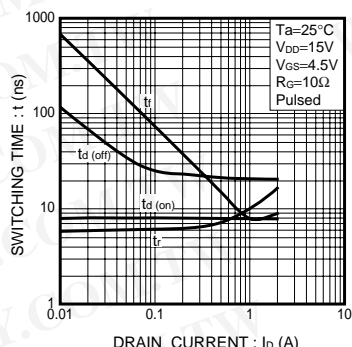
Fig.9 Switching Characteristics
