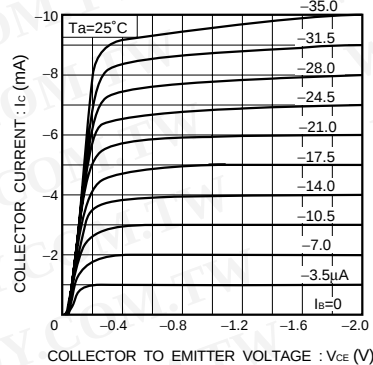
Fig.13 Grounded emitter output characteristics (I)
