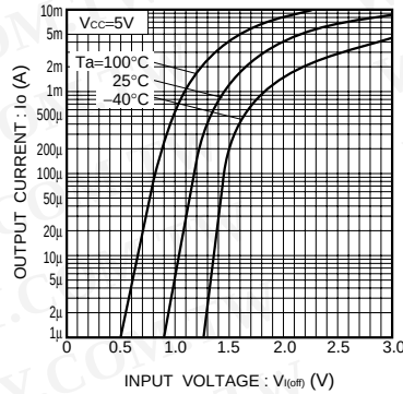
Fig.10 Output current vs. input voltage (OFF characteristics)
