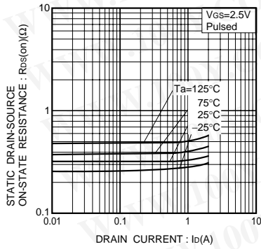
Fig.7 Static Drain-Source On-State Resistance vs. Drain Current(II)
