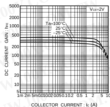
Fig.5 DC current gain vs. collector current (III)
