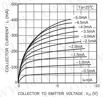
Fig.3 Ground emitter output characteristics (II)
