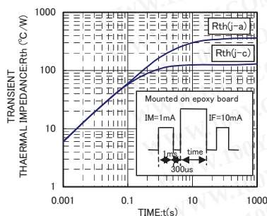
Rth-t CHARACTERISTICS
