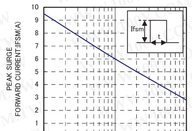
IFSM-t CHARACTERISTICS
