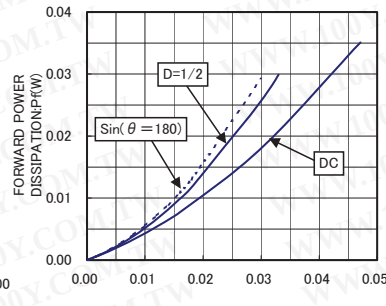
AVERAGE RECTIFIED FORWARD CURRENT Io(A) Io-Pr CHARACTERISTICS
