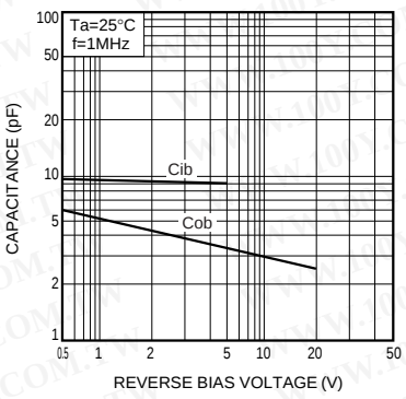
Fig.9 Capacitance vs. reverse bias voltage
