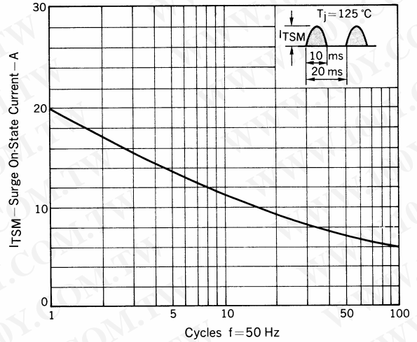
Fig. 10 I_{TSM} RATINGS
