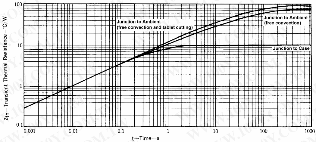
Fig. 11 Z_{th} CHARACTERISTICS
