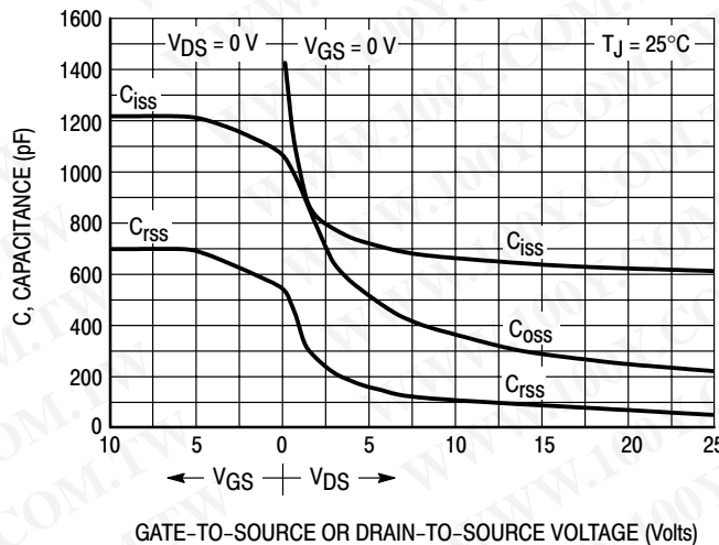
Figure 6. Capacitance Variation
