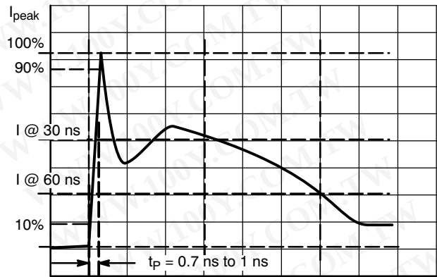
Figure 3. IEC61000-4-2 Spec
