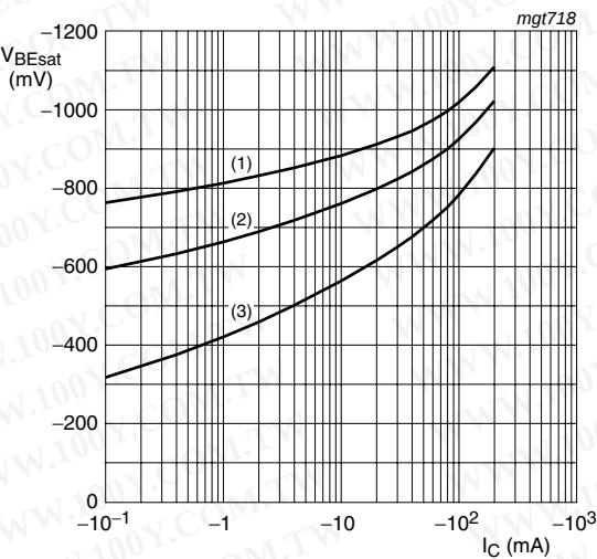
Fig 6. BCV62B: Base-emitter voltage as a function of collector current; typical values
