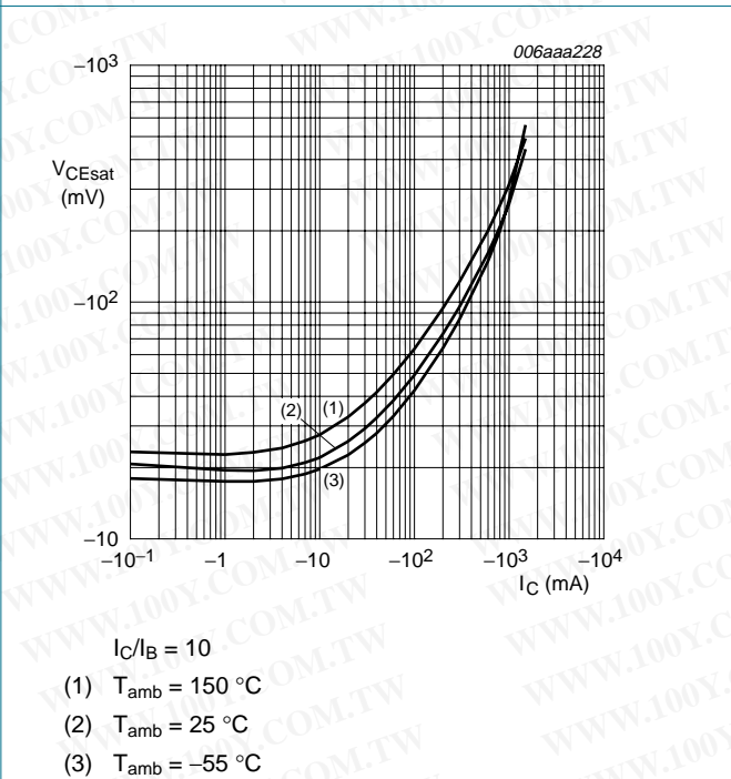
Fig 13. Collector-emitter saturation voltage as a function of collector current; typical values
