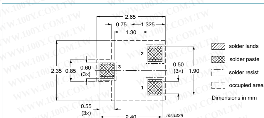
Fig 22. Reflow soldering footprint SOT323 (SC-70)
