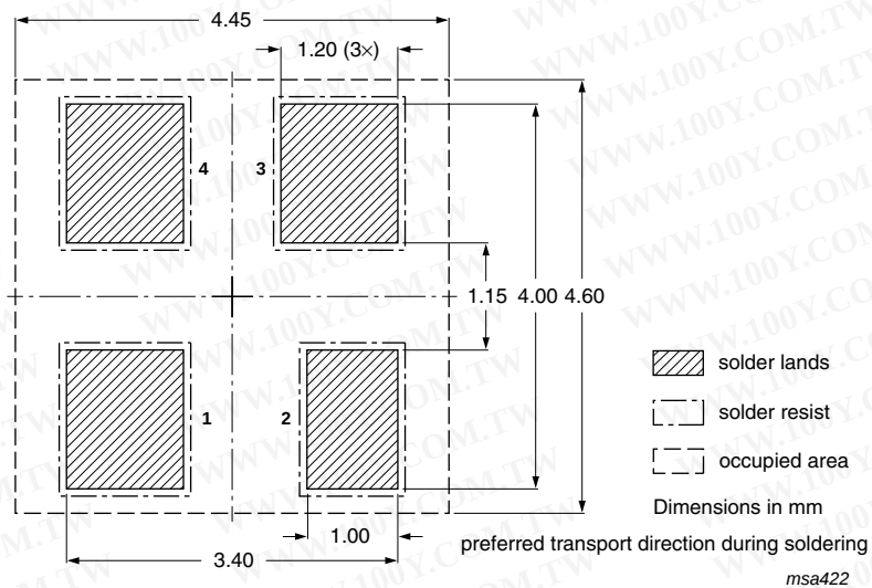
Fig 25. Wave soldering footprint SOT143B
