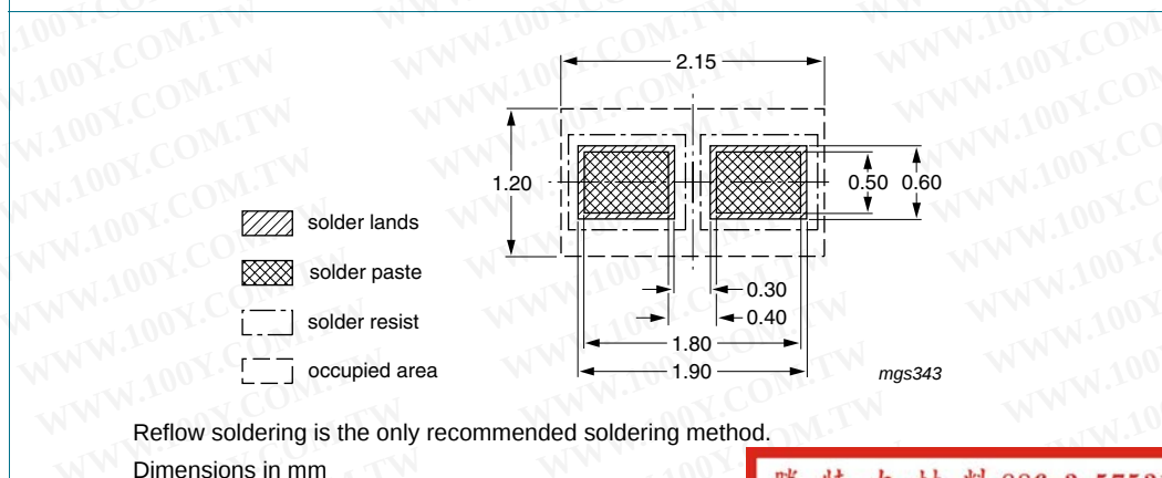
Fig 17. Reflow soldering footprint SOD523 (SC-79)
