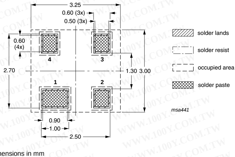
Fig 24. Reflow soldering footprint SOT143B
