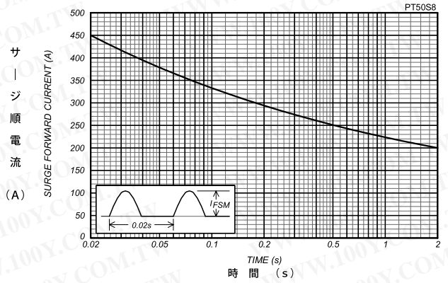
サージ順電流定格 SURGE CURRENT RATINGS f=50Hz, Half Sine Wave, Non-Repetitive, Tj=150°C
