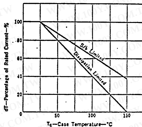
OPERATING CURVE OF SAFE OPERATING AREA
