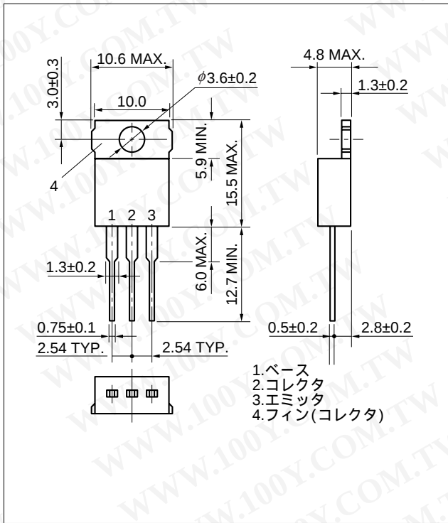
TO-220AB (MP-25)
